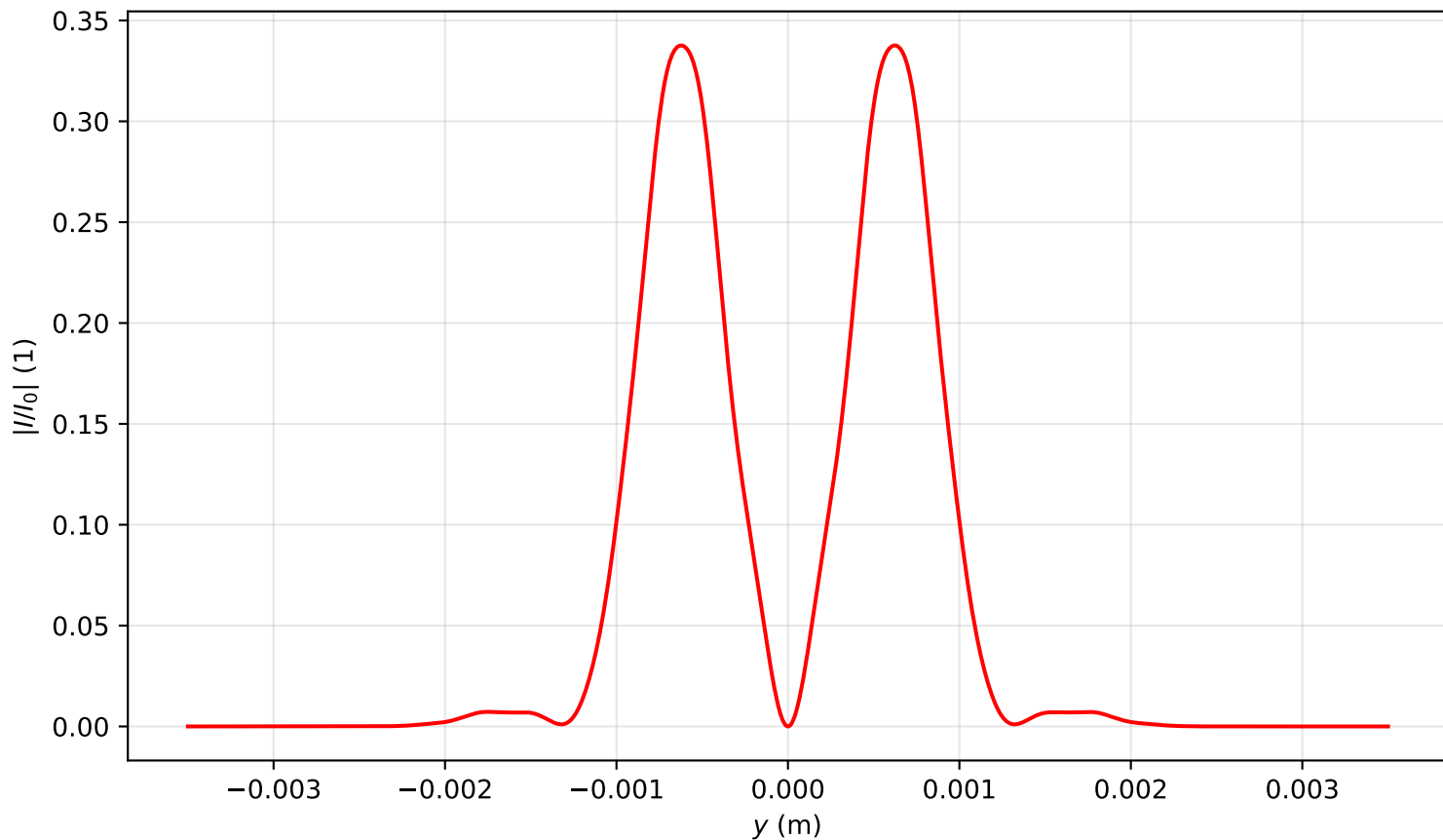
Intensity profile I(x=0, y, z=1.592)/I_0 , P_{in}=5.0P_{cr} , artificial time
